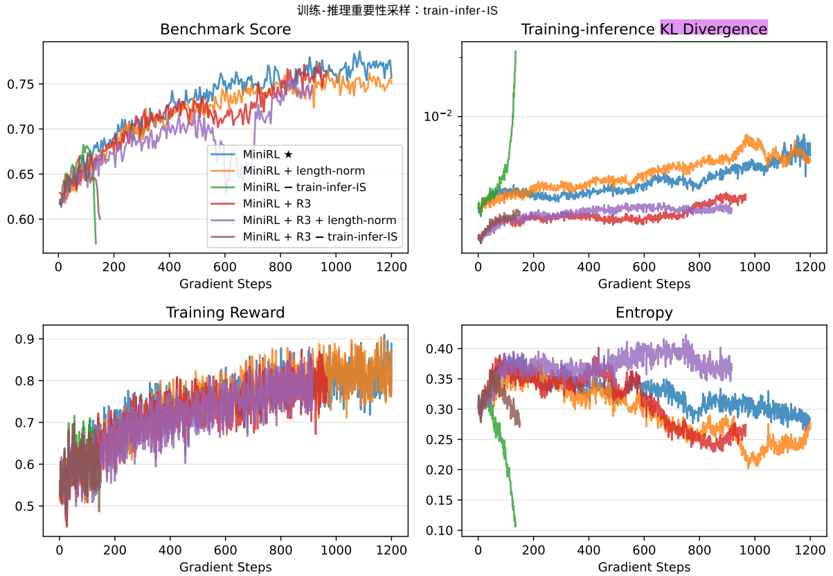
Figure 1: Results of on-policy training with gbs (global batch size) = mbs (mini-batch size) = 1,024.
