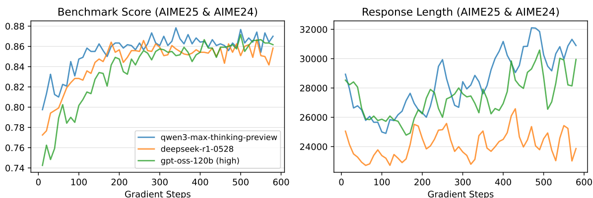
Figure 5: Results of varying cold-start initializations.
