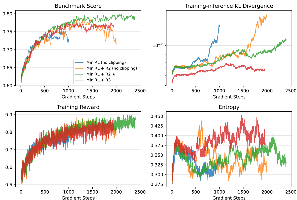
Figure 2: Results of off-policy training with gbs = 2 \times mbs = 2,048 .
